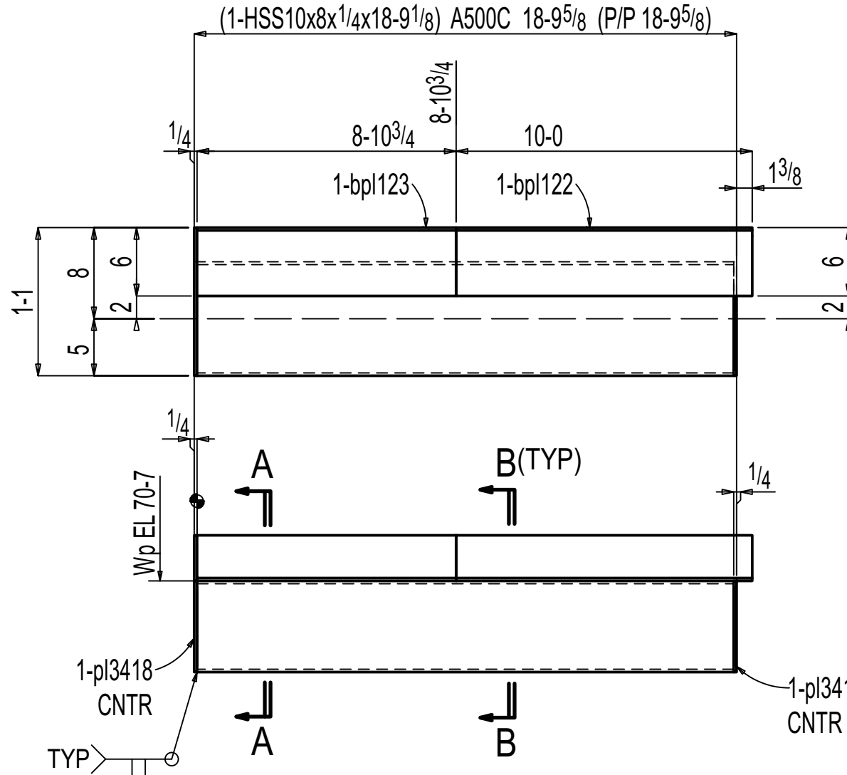
ONE BEAM F-09.03B1
